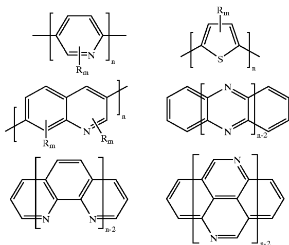
Scheme 3 Heterocyclic/fused ring heterocyclic combinations
