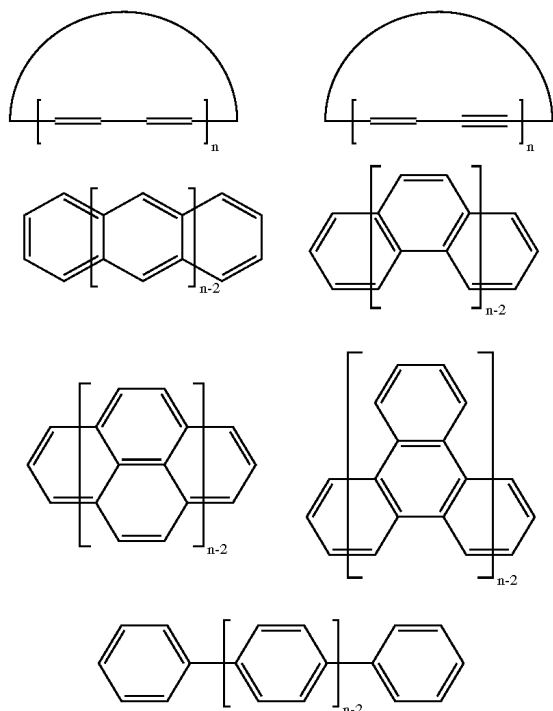
Scheme 2 Cyclic and fused ring combinations.
