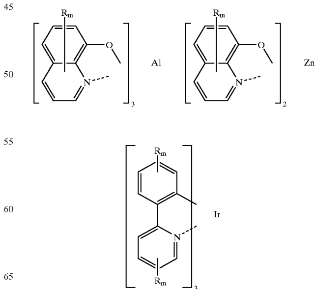
Scheme 4 Metal complexed organo-metallic compounds. (R: D, H, C_1-C_{30} alkoxyl, C_1-C_{30} silyl, aryl, heteroaryl; m is 1-4).
