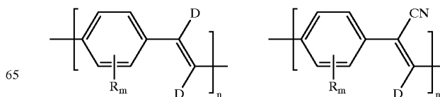
Scheme 5 Organic semiconductor compounds and polymers with deuterium substituents. (R: D, H, C 1 -C 30 alkyl, C 1 -C 30 alkoxy, phenyl, thienyl, pyridyl, C 1 -C 30 silyl, aryl, heteroaryl; m is from 1 to 4).
