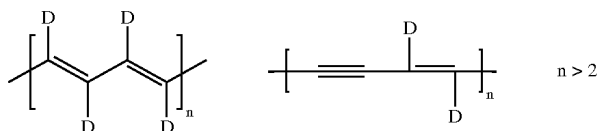
Scheme 1 Linear conjugated organic compounds and polymers
